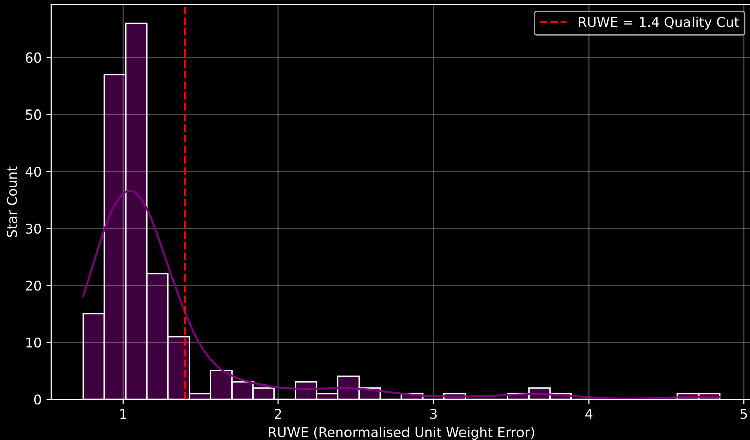
GAPOGEE DR17 Field [161-57] RUWE Distribution (n= 200)
