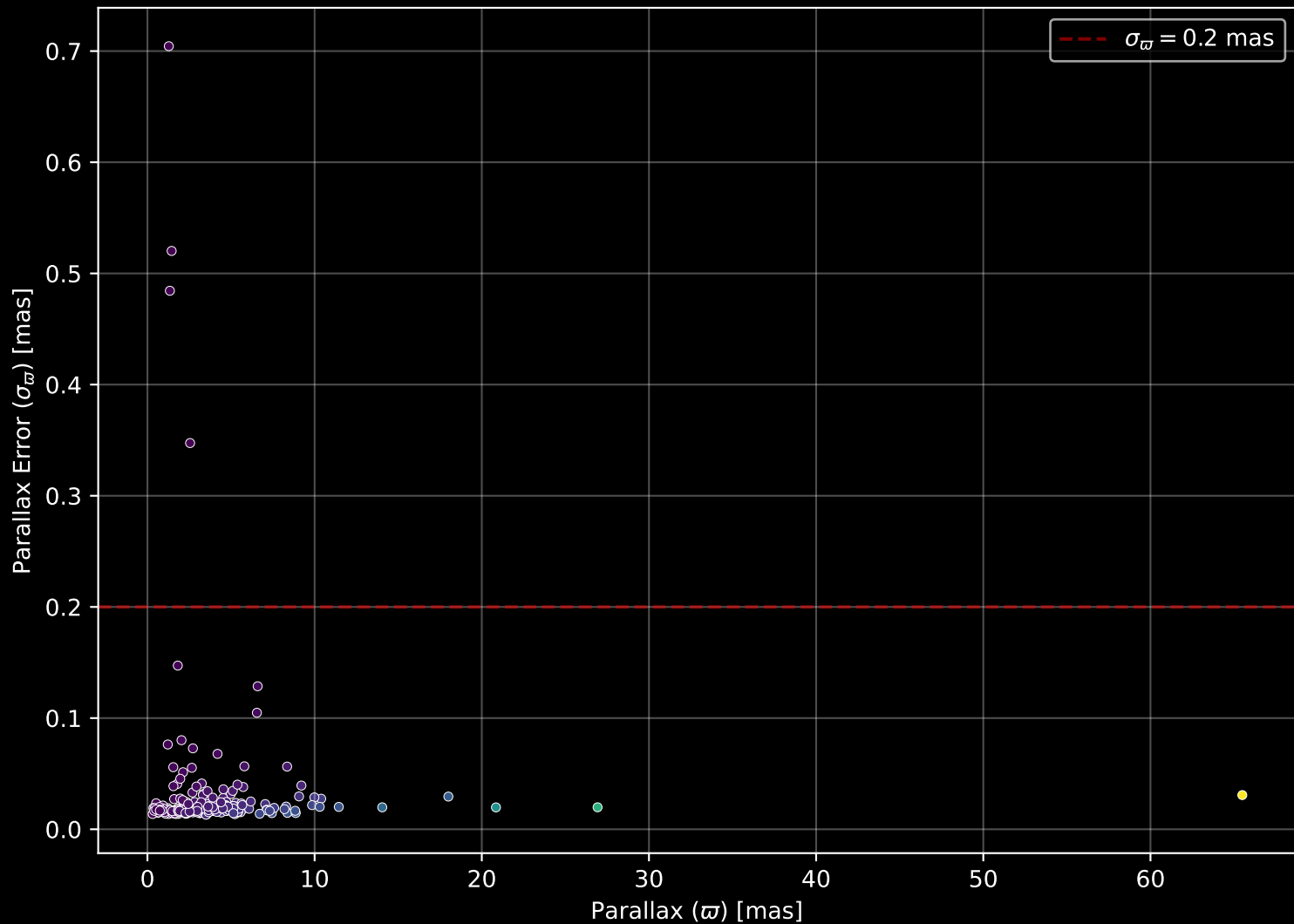
APOGEE DR17 Field: [161-57] Parallax Quality (n= 207)
