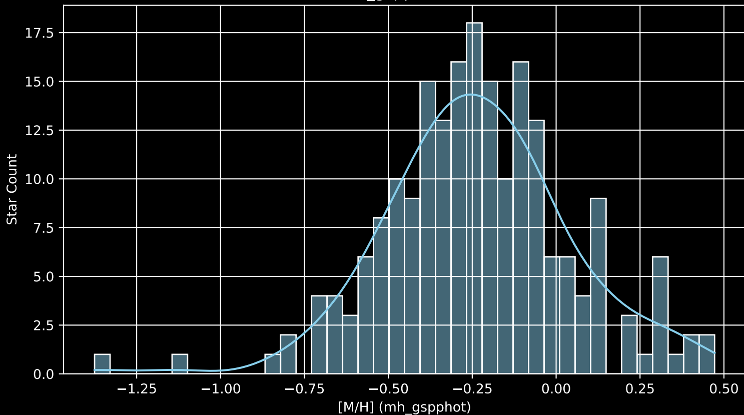
APOGEE DR17 Field: [161-57 [M/H] (mh_gspphot) (n= 205)
