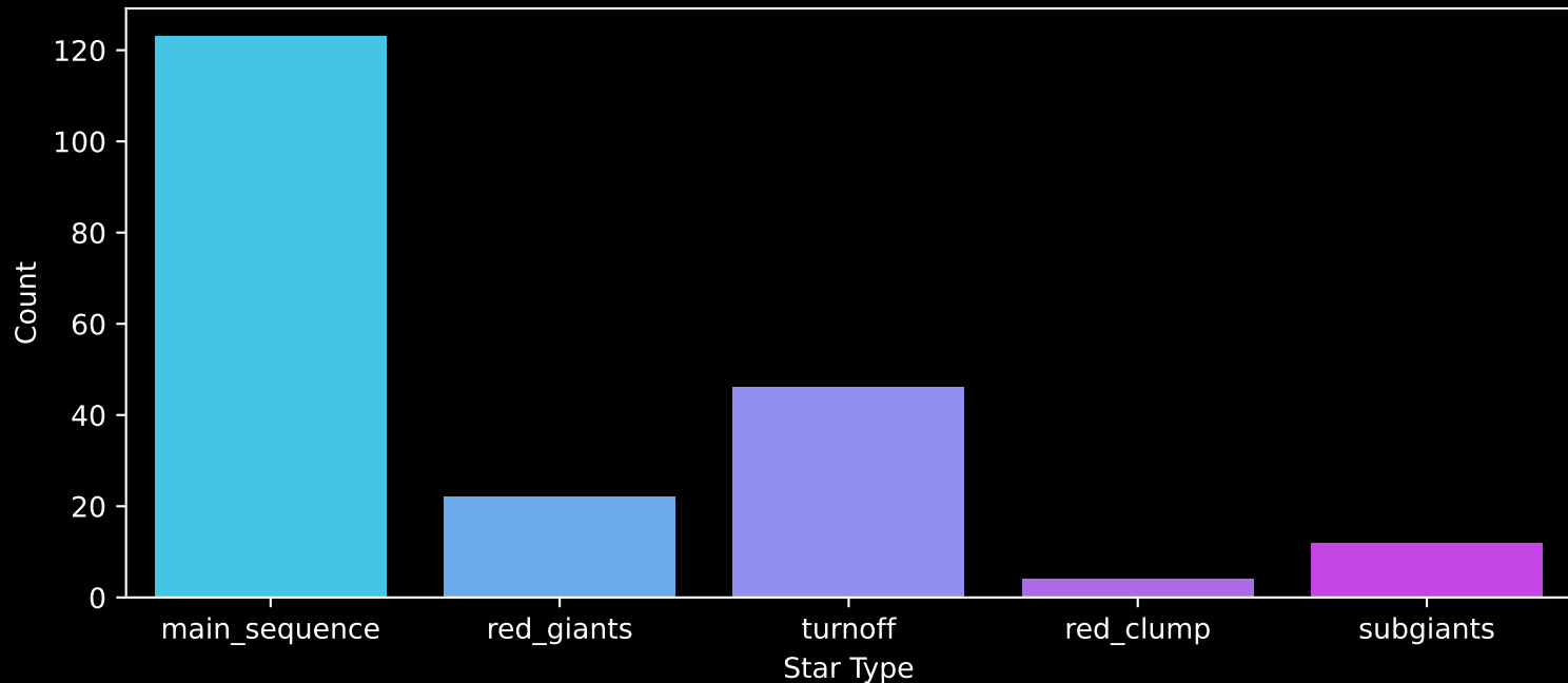
APOGEE DR17 Field: [161-57] Count plot of Star Type
