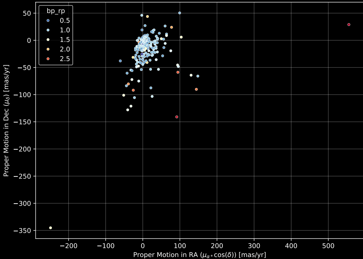
APOGEE DR17 Field: [161-57] Proper Motion Diagram (n= 207)
