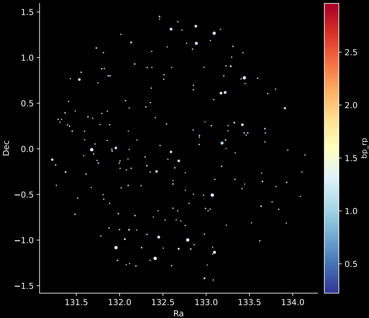
APOGEE DR17 Field: [161-57] Stars: 207
